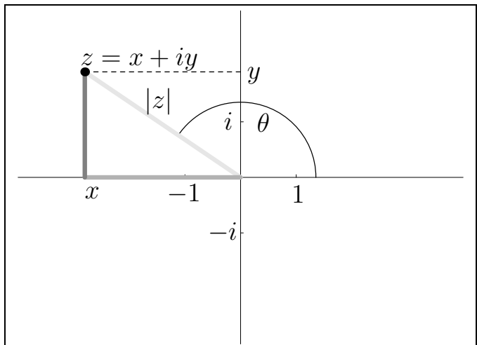
Fig. 4: x < 0, y > 0, \pi/2 < \theta < \pi
