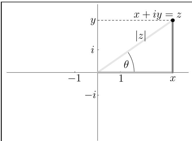
Fig. 3: x > 0, y > 0, 0 < \theta < \pi/2
