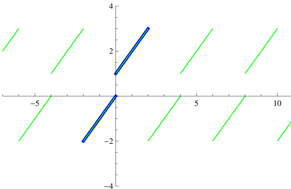
The Fourier sine series
