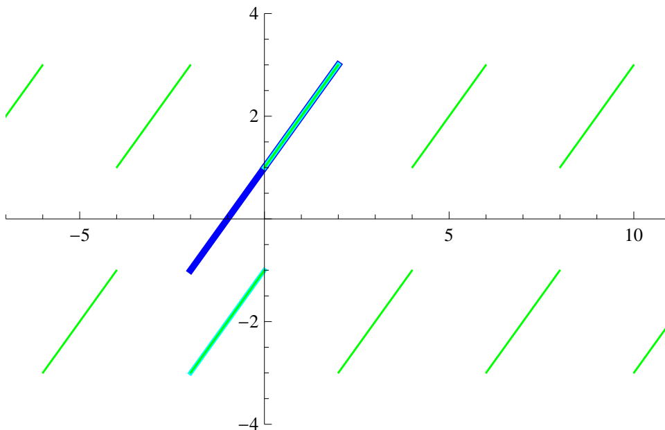
The Fourier cosine series
