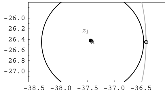
FIGURE 4. A zoom-in on z_1 with a root of z^5 - 45^5 marked by a gray disk
